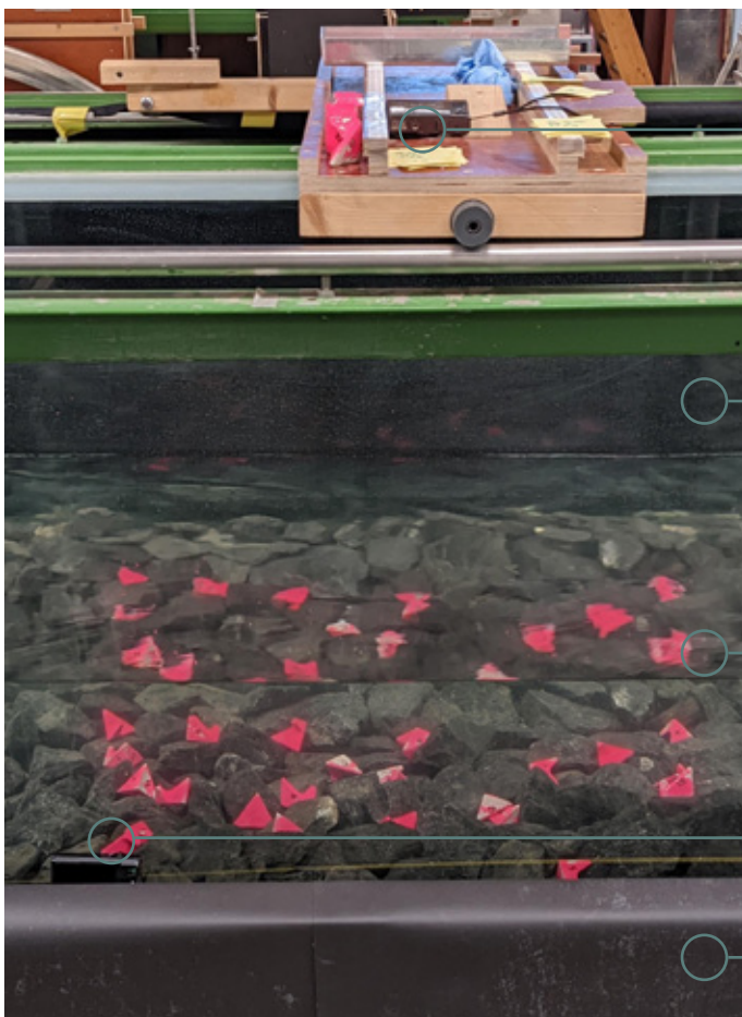
Figure 55: Camera setup.
